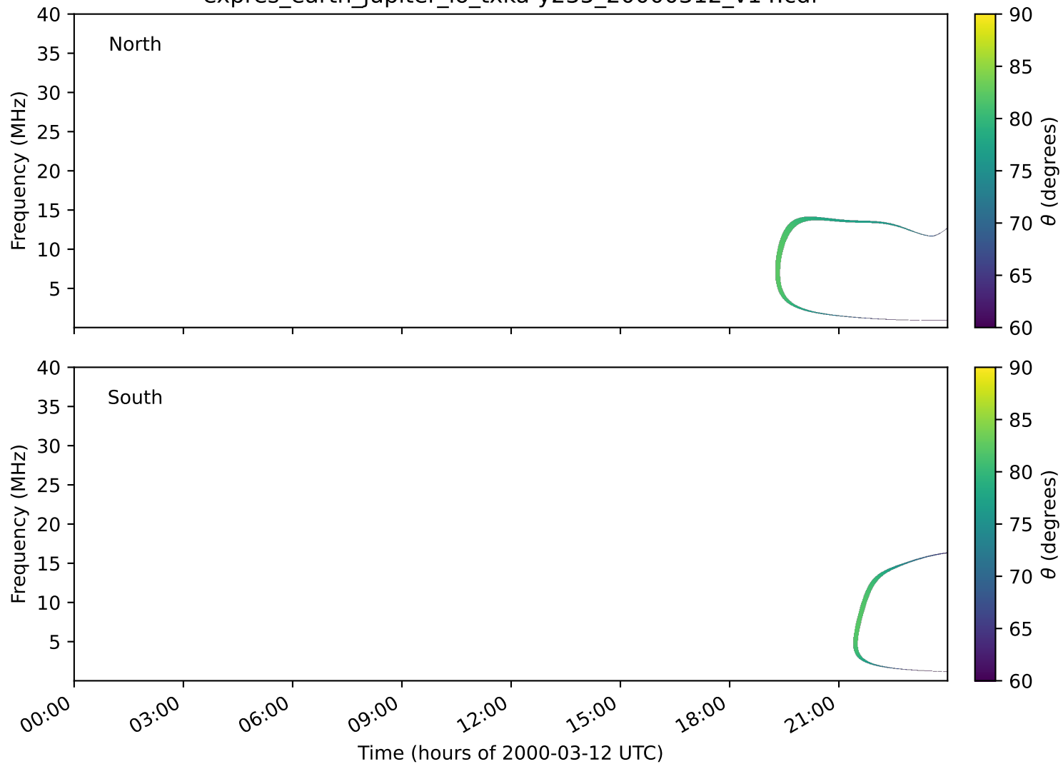
expres_earth_jupiter_io_txka-y235_20000312_v14.cdf
