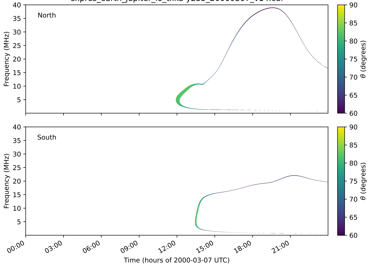
expres_earth_jupiter_io_txka-y235_20000307_v14.cdf
