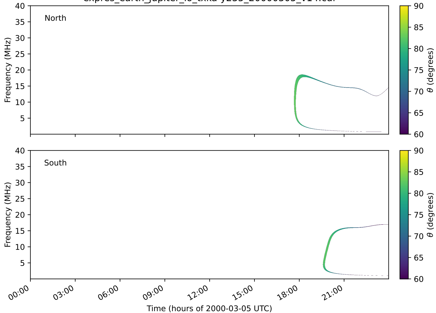
expres_earth_jupiter_io_txka-y235_20000305_v14.cdf
