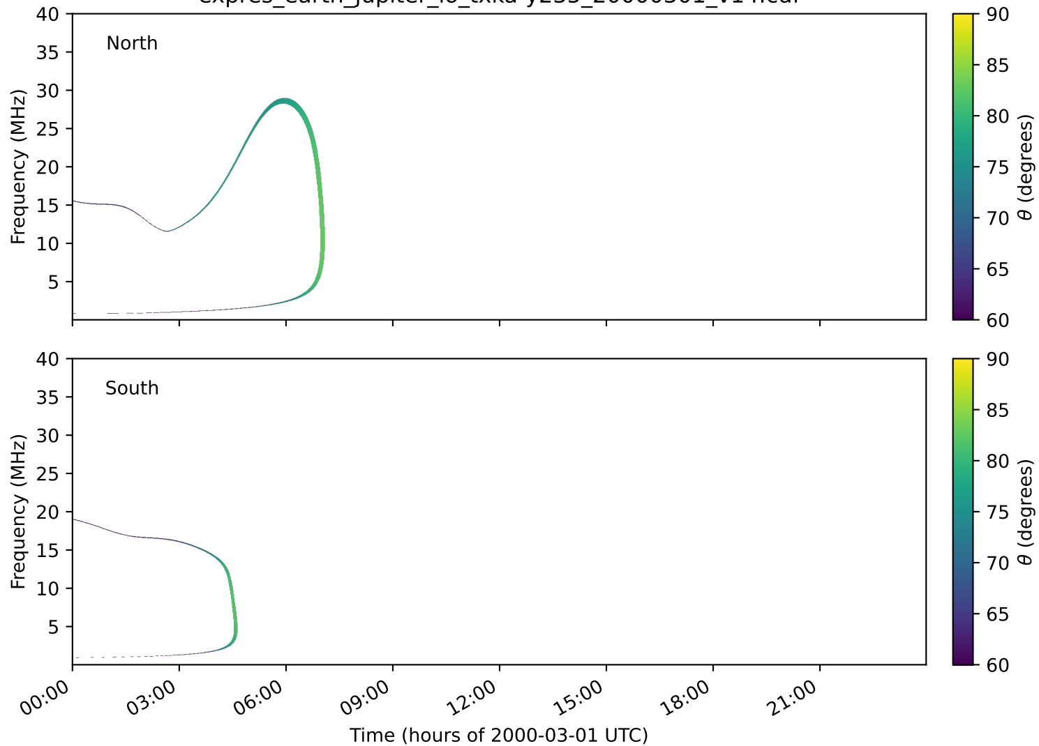
expres_earth_jupiter_io_txka-y235_20000301_v14.cdf
