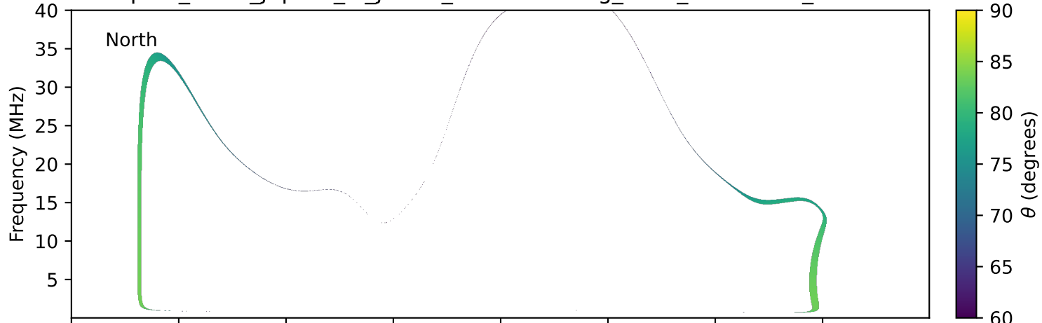
expres_earth_jupiter_io_jrm33_lossc-wid1deg_3kev_20000311_v11.cdf
