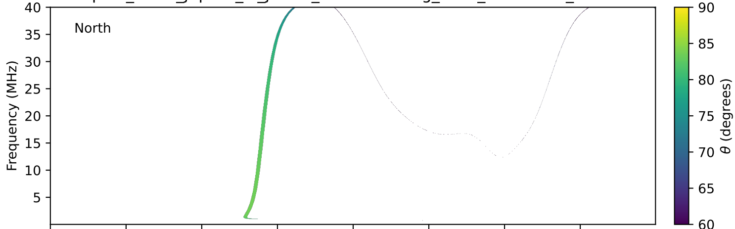
expres_earth_jupiter_io_jrm33_lossc-wid1deg_3kev_20000309_v11.cdf
