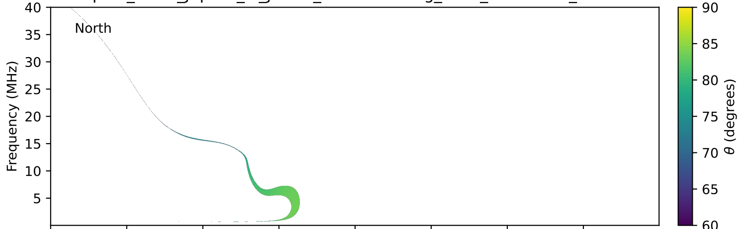
expres_earth_jupiter_io_jrm09_lossc-wid1deg_3kev_20000331_v11.cdf
