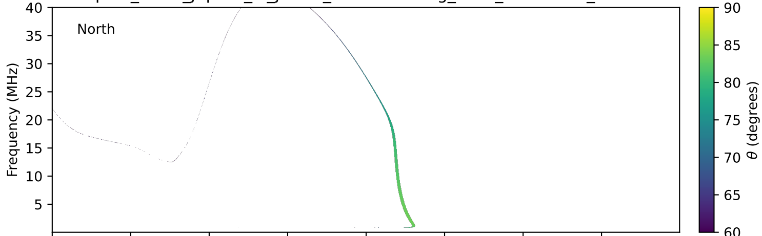
expres_earth_jupiter_io_jrm09_lossc-wid1deg_3kev_20000329_v11.cdf
