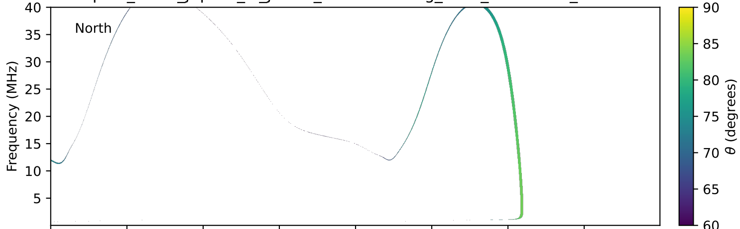
expres_earth_jupiter_io_jrm09_lossc-wid1deg_3kev_20000320_v11.cdf
