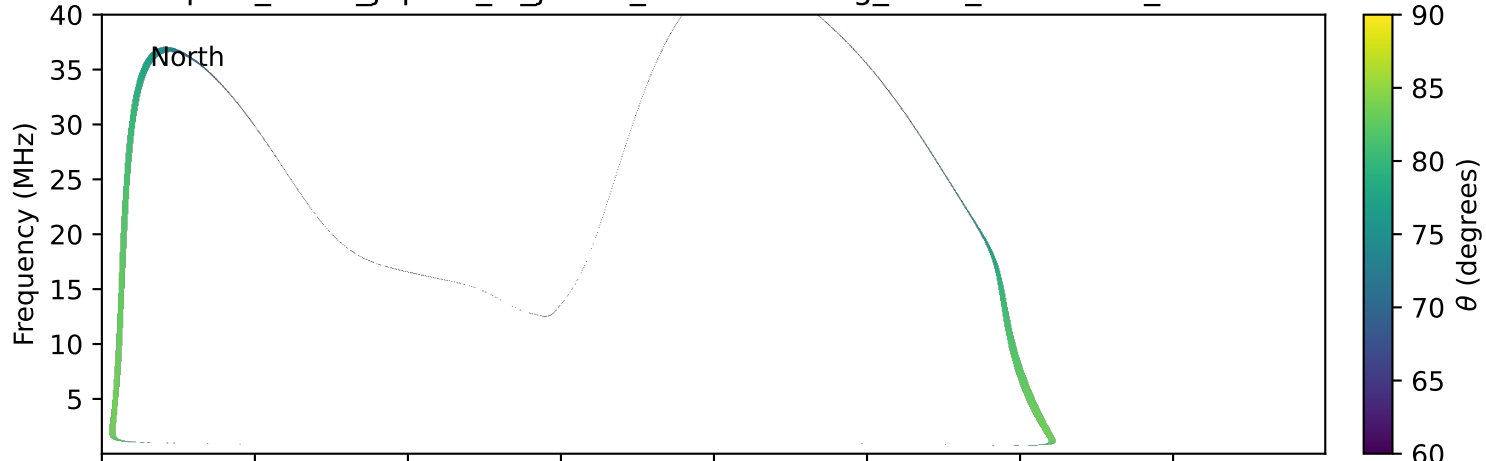
expres_earth_jupiter_io_jrm09_lossc-wid1deg_3kev_20000304_v11.cdf
