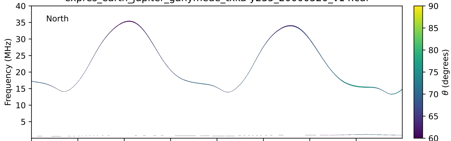
expres_earth_jupiter_ganymede_txka-y235_20000320_v14.cdf
