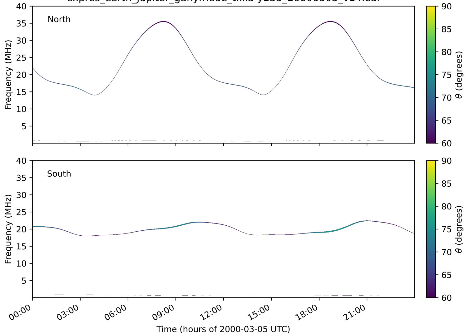
expres_earth_jupiter_ganymede_txka-y235_20000305_v14.cdf
