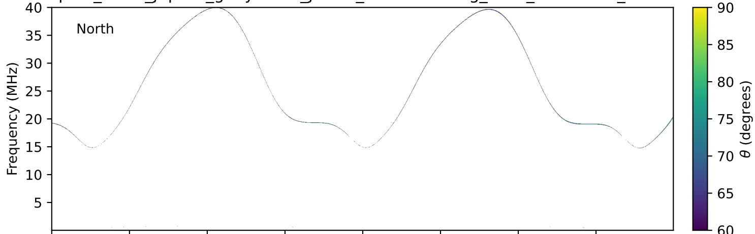
expres_earth_jupiter_ganymede_jrm33_lossc-wid1deg_3kev_20000320_v11.cdf
