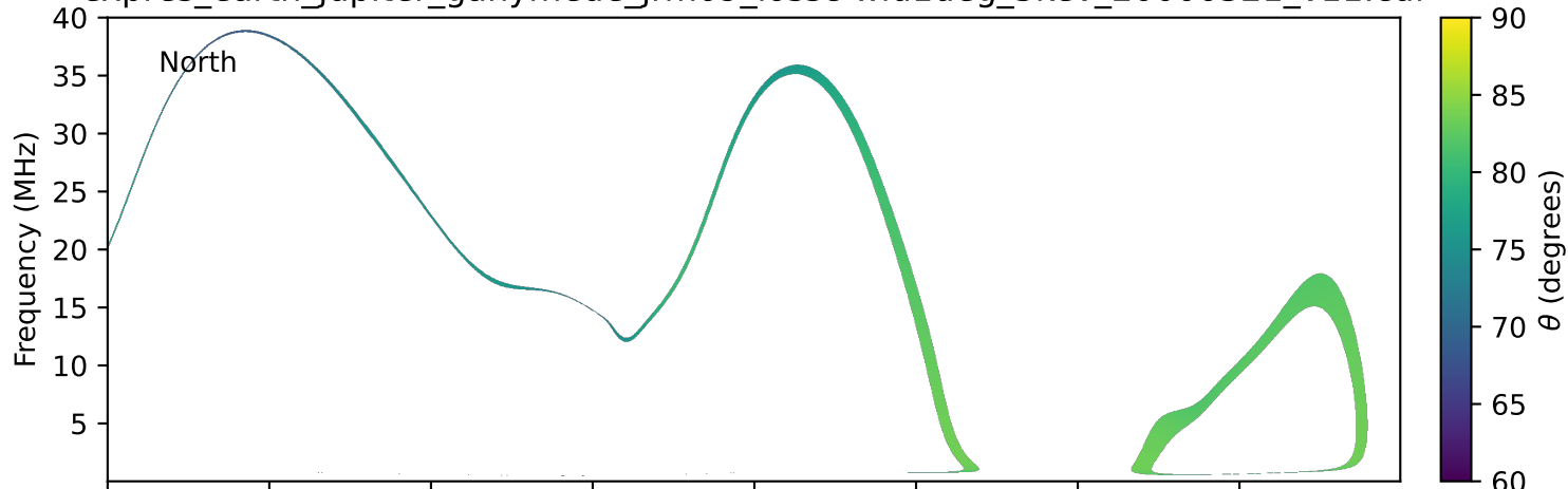
expres_earth_jupiter_ganymede_jrm09_lossc-wid1deg_3kev_20000321_v11.cdf
