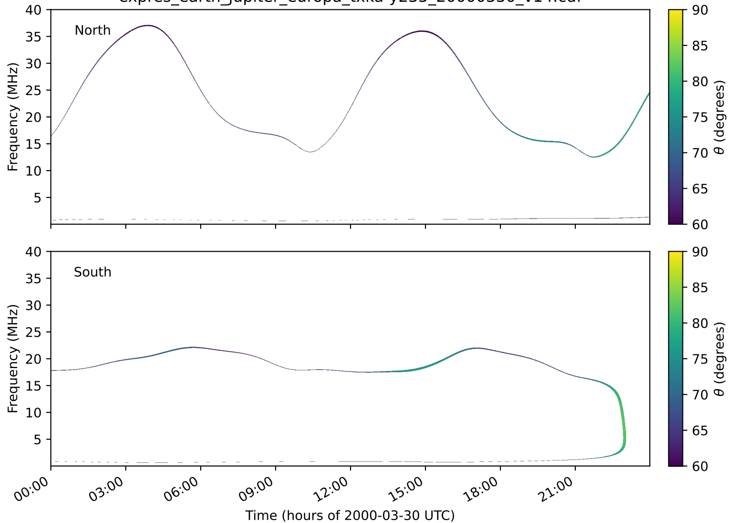
expres_earth_jupiter_europa_txka-y235_20000330_v14.cdf
