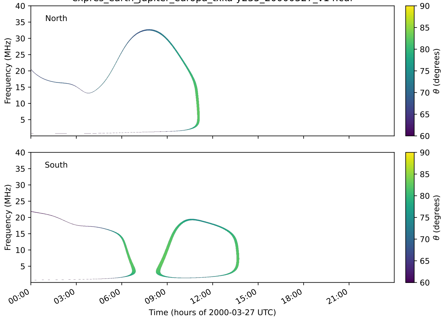
expres_earth_jupiter_europa_txka-y235_20000327_v14.cdf
