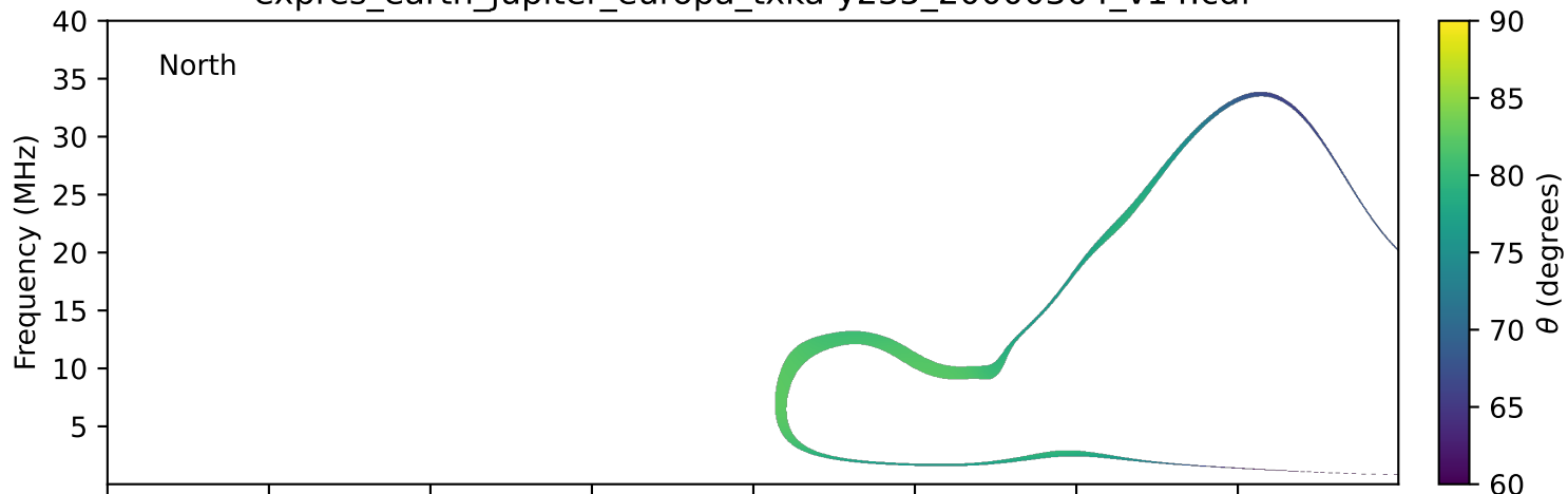
expres_earth_jupiter_europa_txka-y235_20000304_v14.cdf
