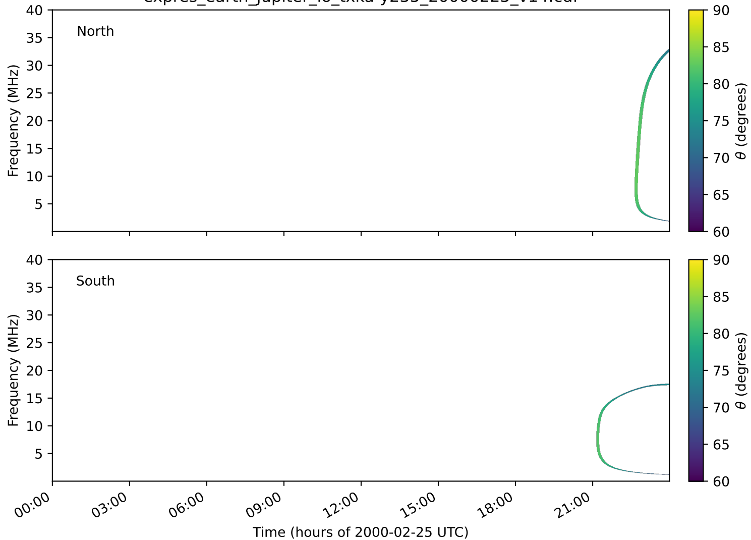
expres_earth_jupiter_io_txka-y235_20000225_v14.cdf
