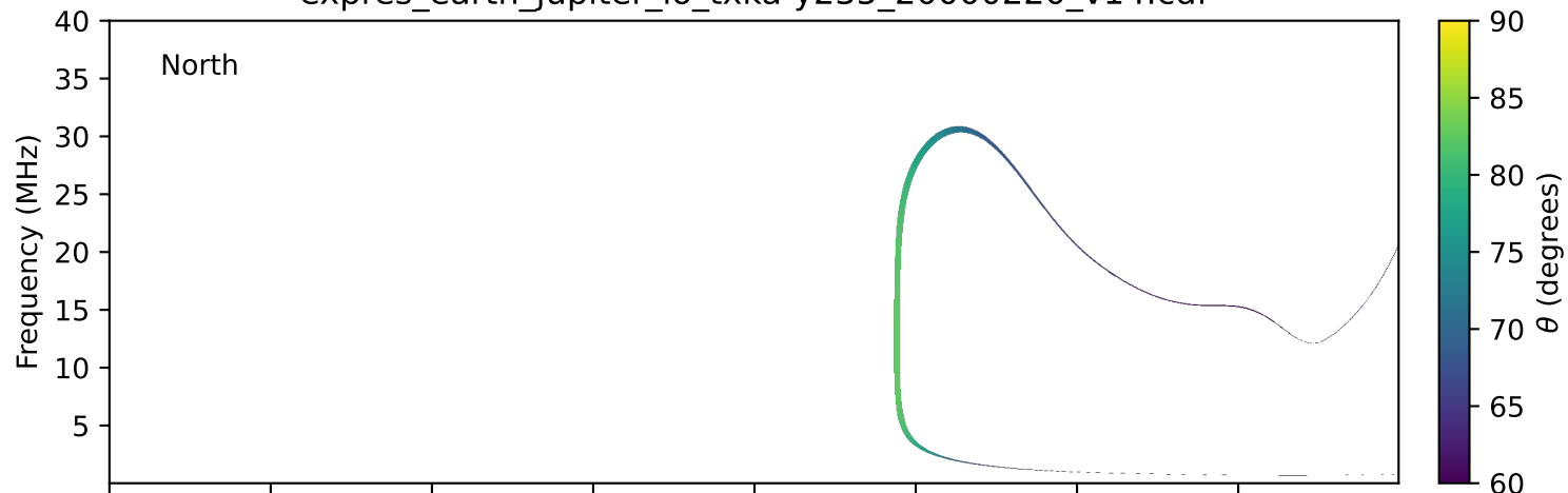
expres_earth_jupiter_io_txka-y235_20000220_v14.cdf
