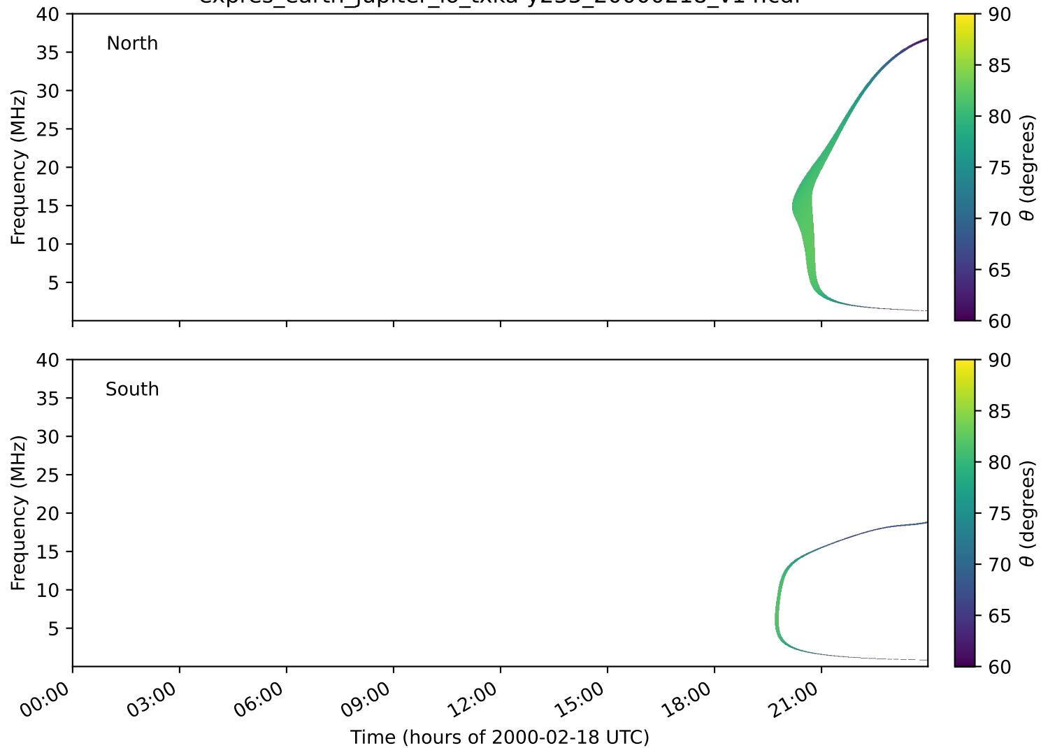
expres_earth_jupiter_io_txka-y235_20000218_v14.cdf
