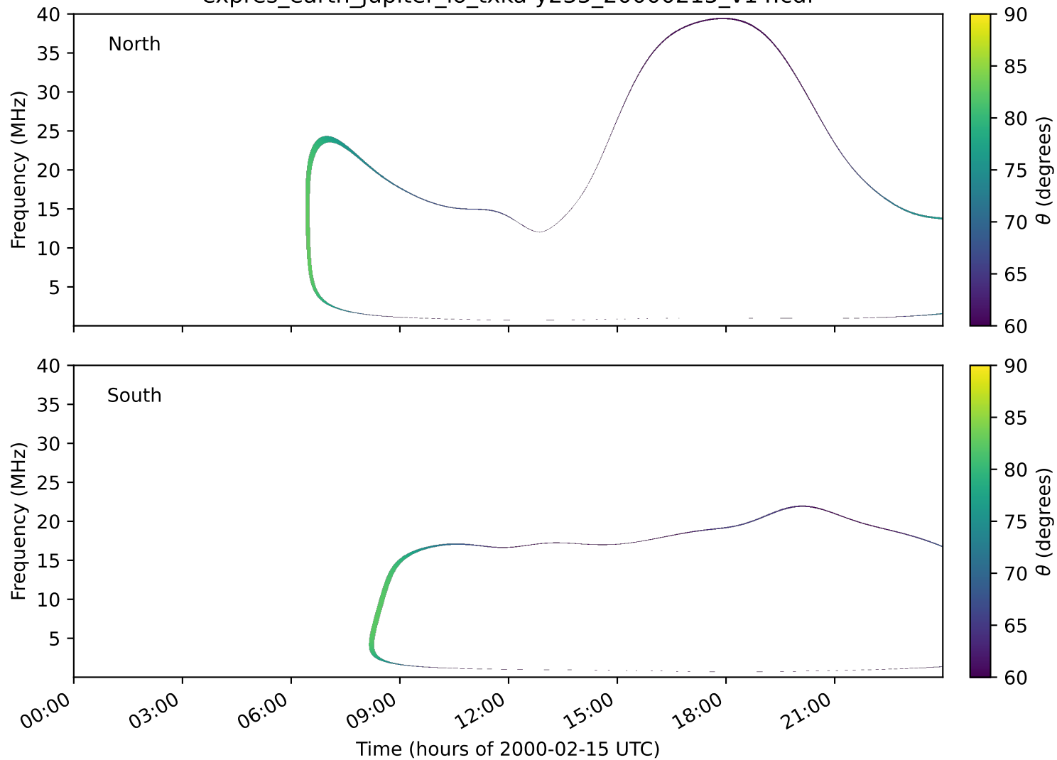
expres_earth_jupiter_io_txka-y235_20000215_v14.cdf
