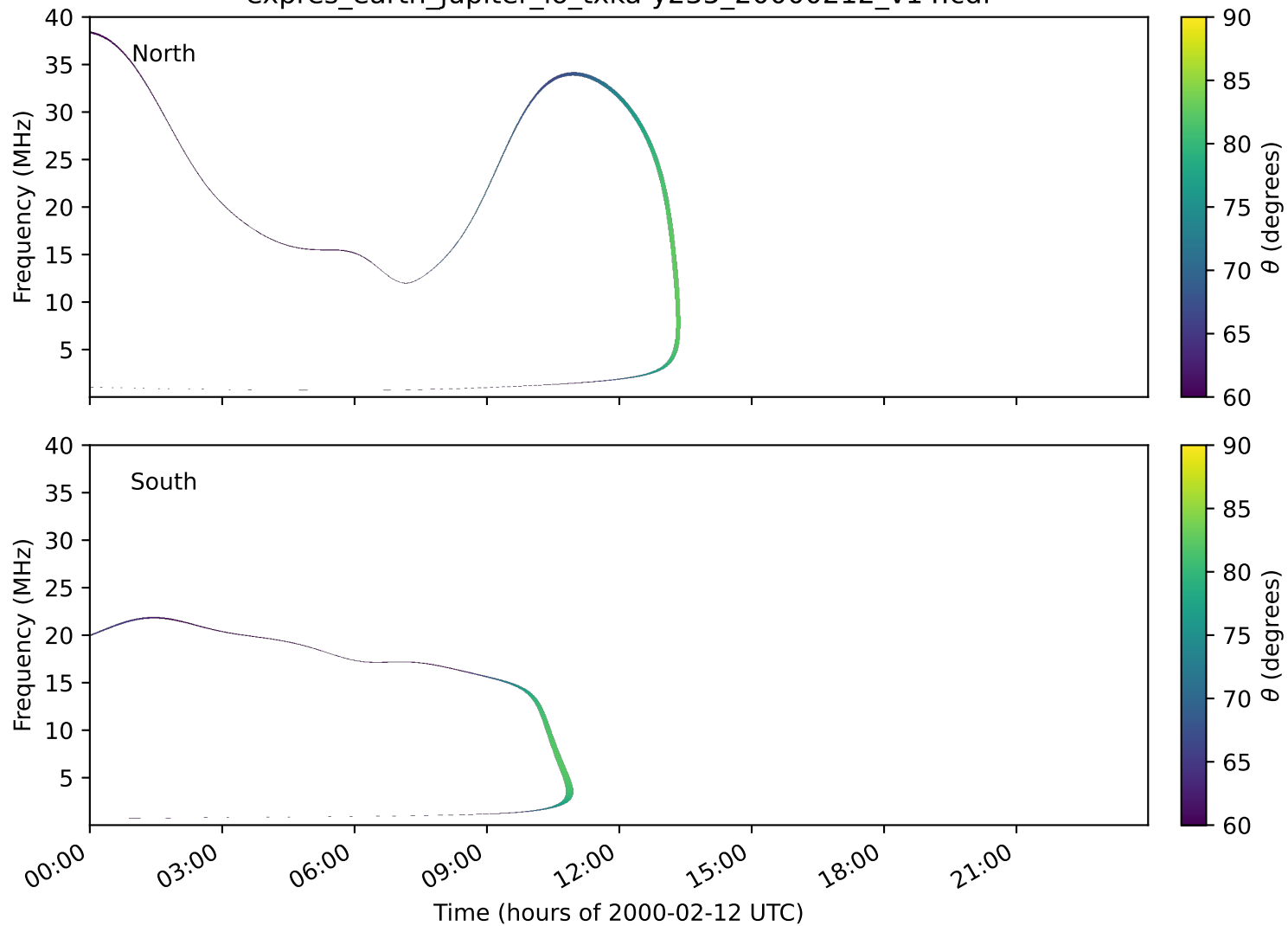
expres_earth_jupiter_io_txka-y235_20000212_v14.cdf
