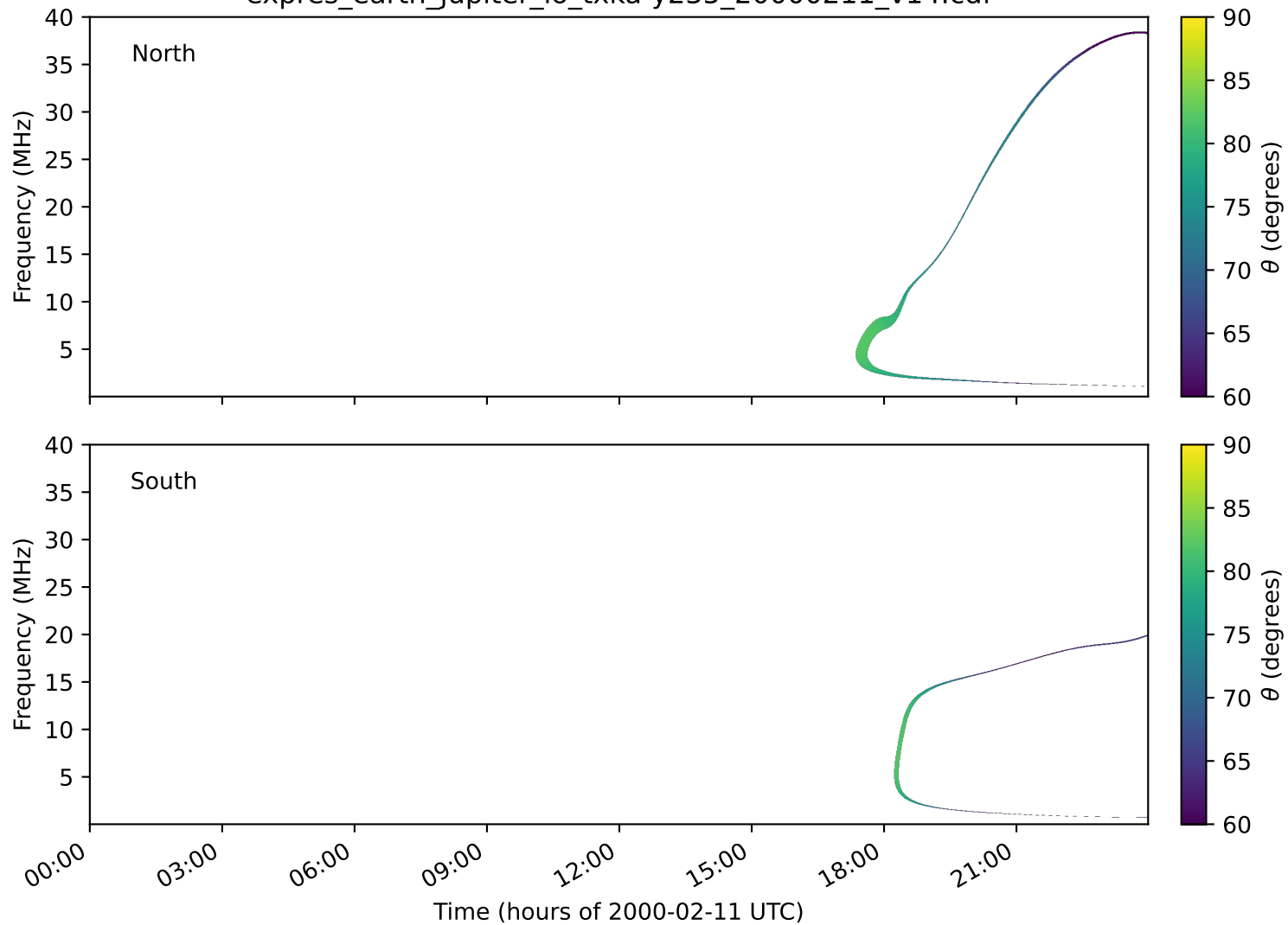
expres_earth_jupiter_io_txka-y235_20000211_v14.cdf
