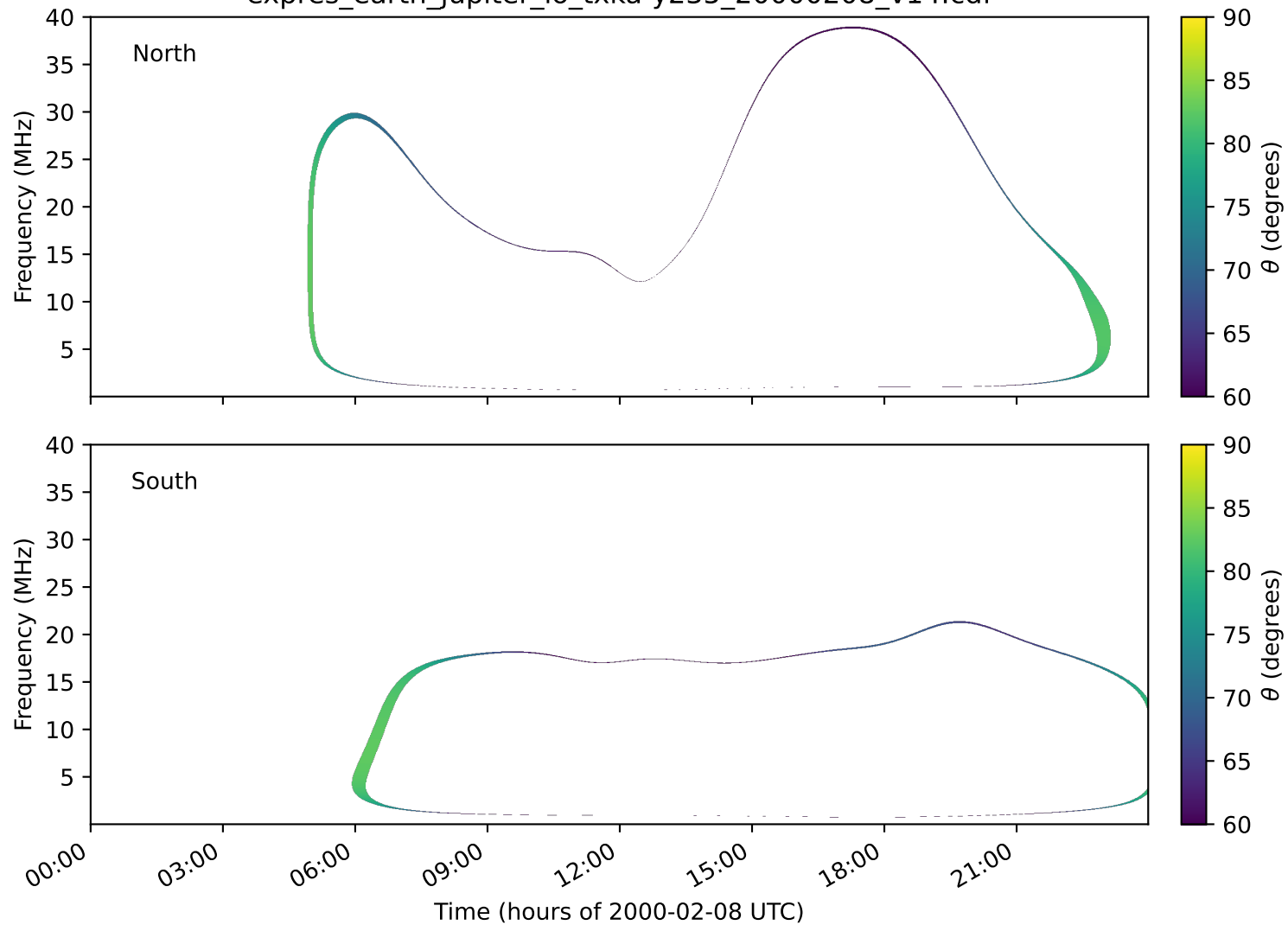
expres_earth_jupiter_io_txka-y235_20000208_v14.cdf
