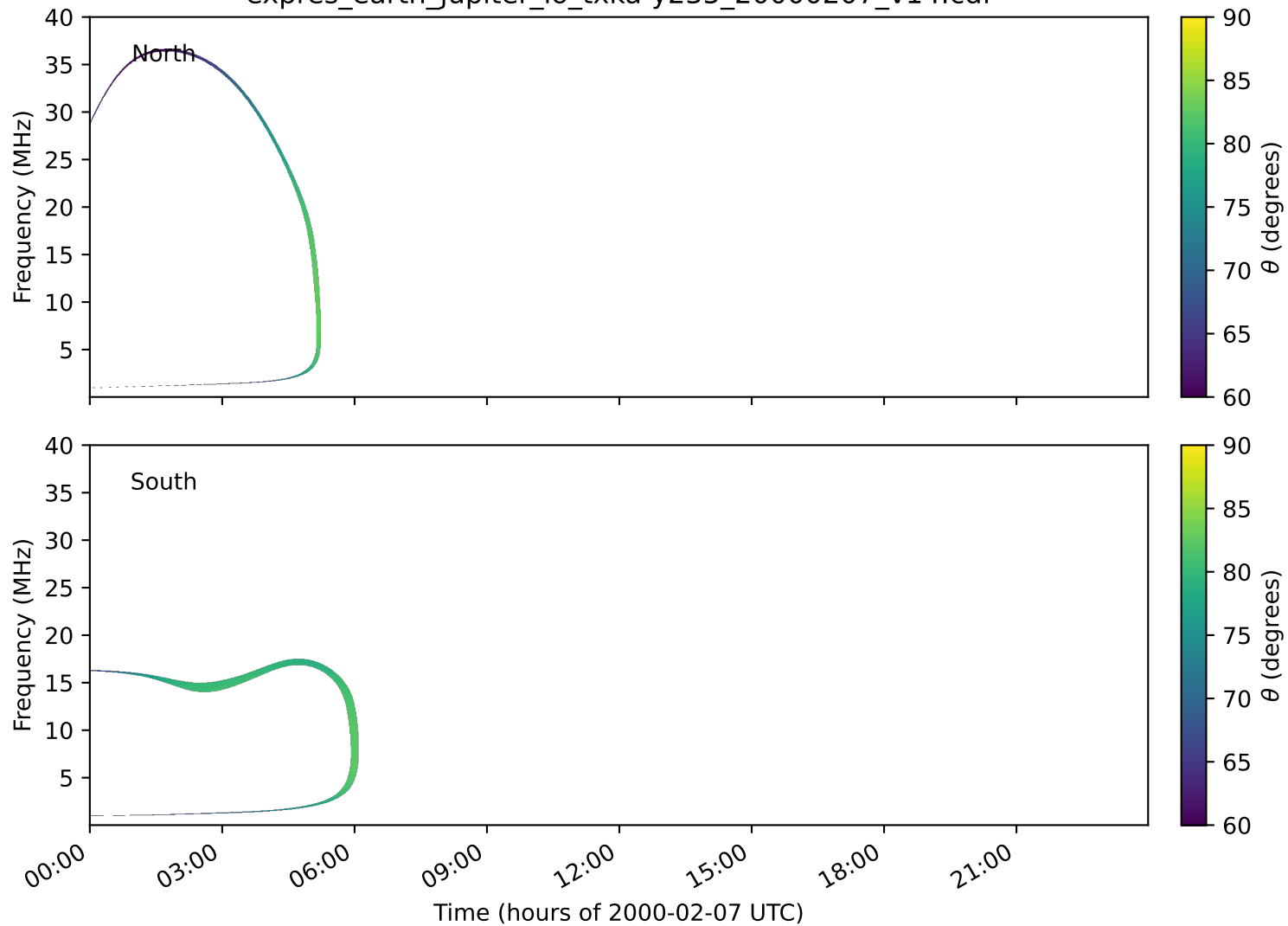
expres_earth_jupiter_io_txka-y235_20000207_v14.cdf
