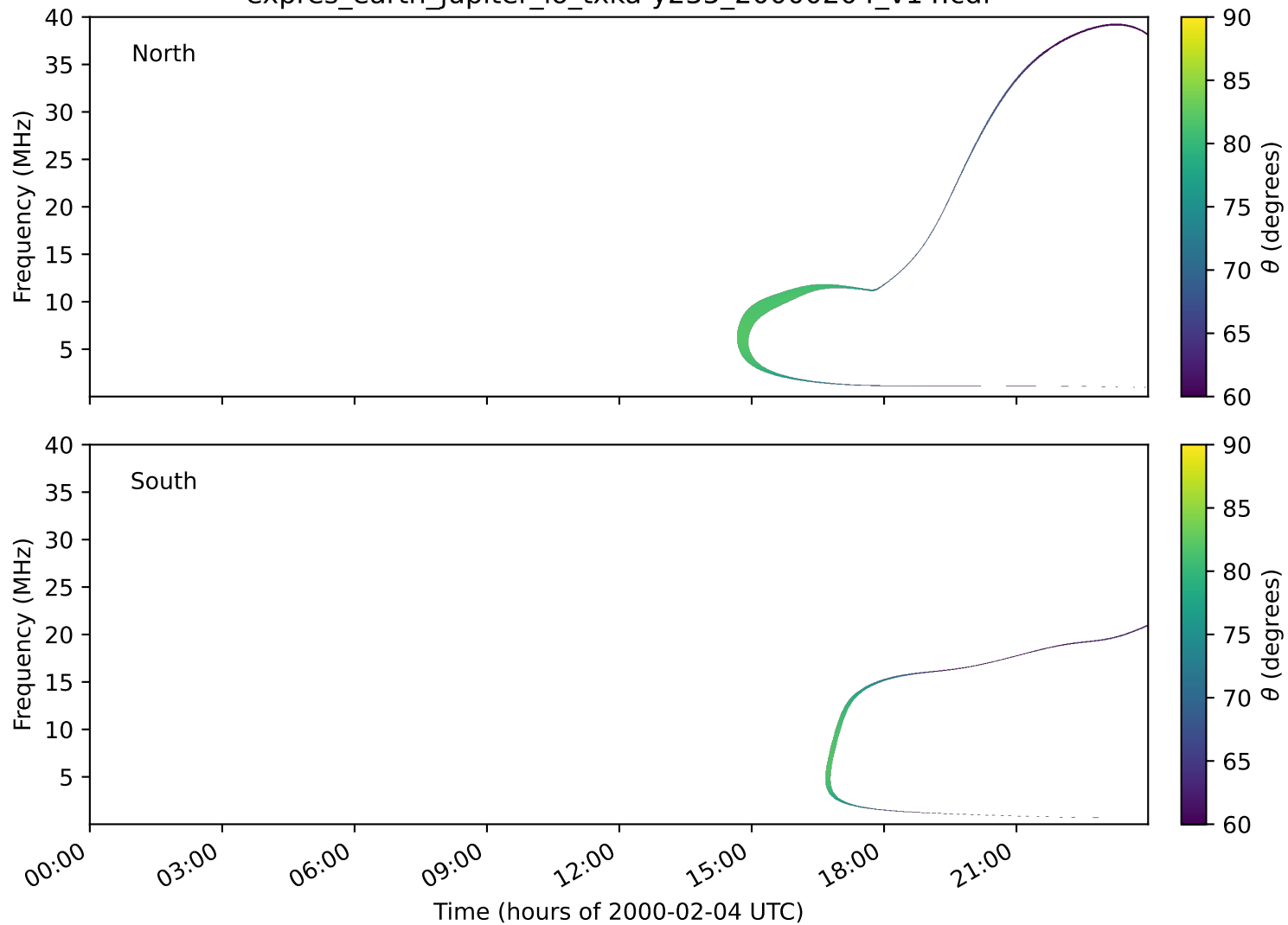
expres_earth_jupiter_io_txka-y235_20000204_v14.cdf
