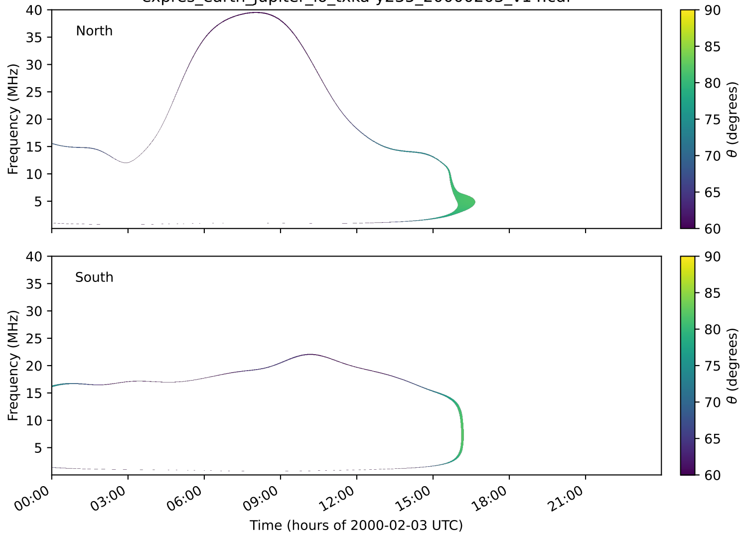
expres_earth_jupiter_io_txka-y235_20000203_v14.cdf
