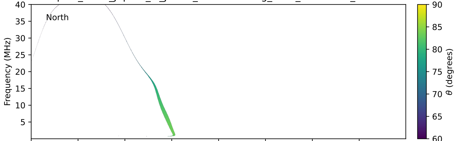
expres_earth_jupiter_io_jrm33_lossc-wid1deg_3kev_20000221_v11.cdf
