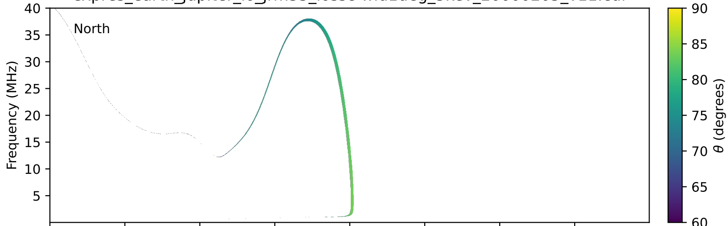
expres_earth_jupiter_io_jrm33_lossc-wid1deg_3kev_20000205_v11.cdf
