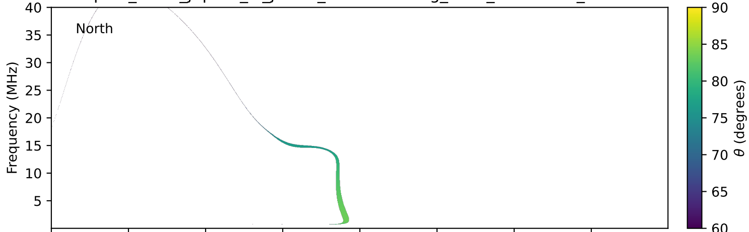
expres_earth_jupiter_io_jrm09_lossc-wid1deg_3kev_20000228_v11.cdf
