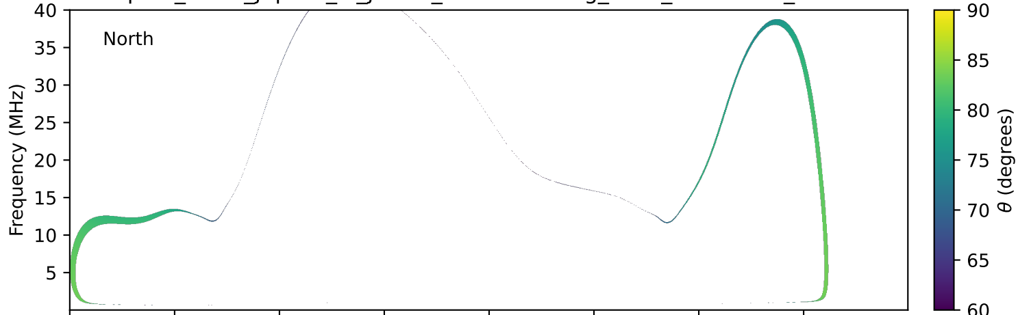
expres_earth_jupiter_io_jrm09_lossc-wid1deg_3kev_20000217_v11.cdf
