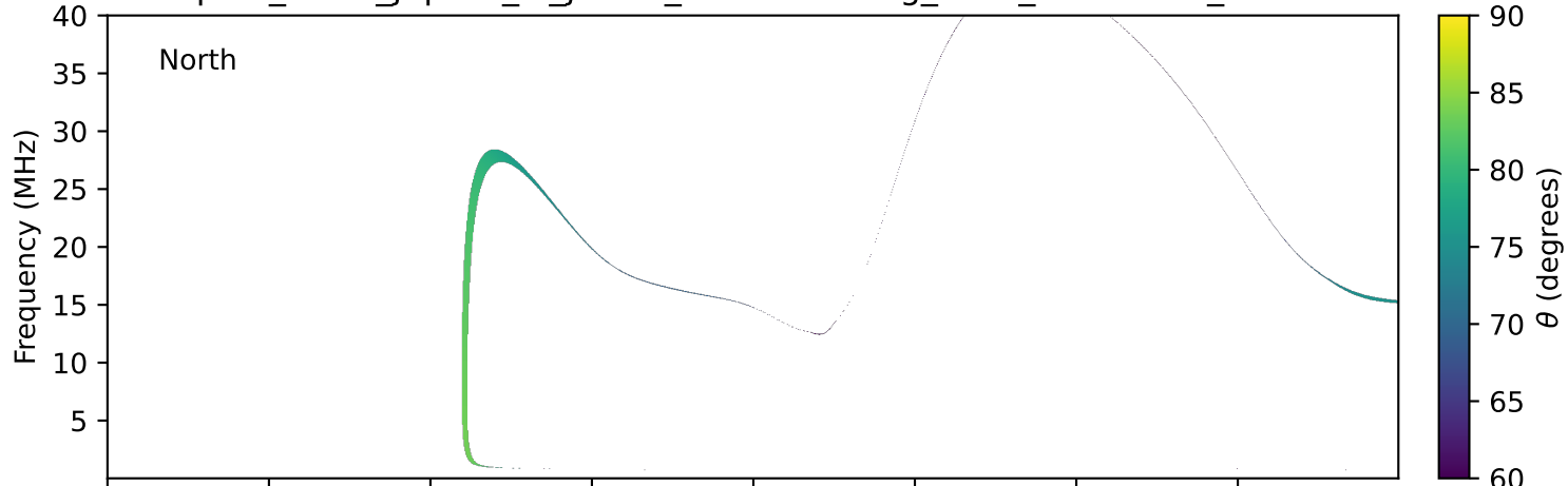
expres_earth_jupiter_io_jrm09_lossc-wid1deg_3kev_20000215_v11.cdf
