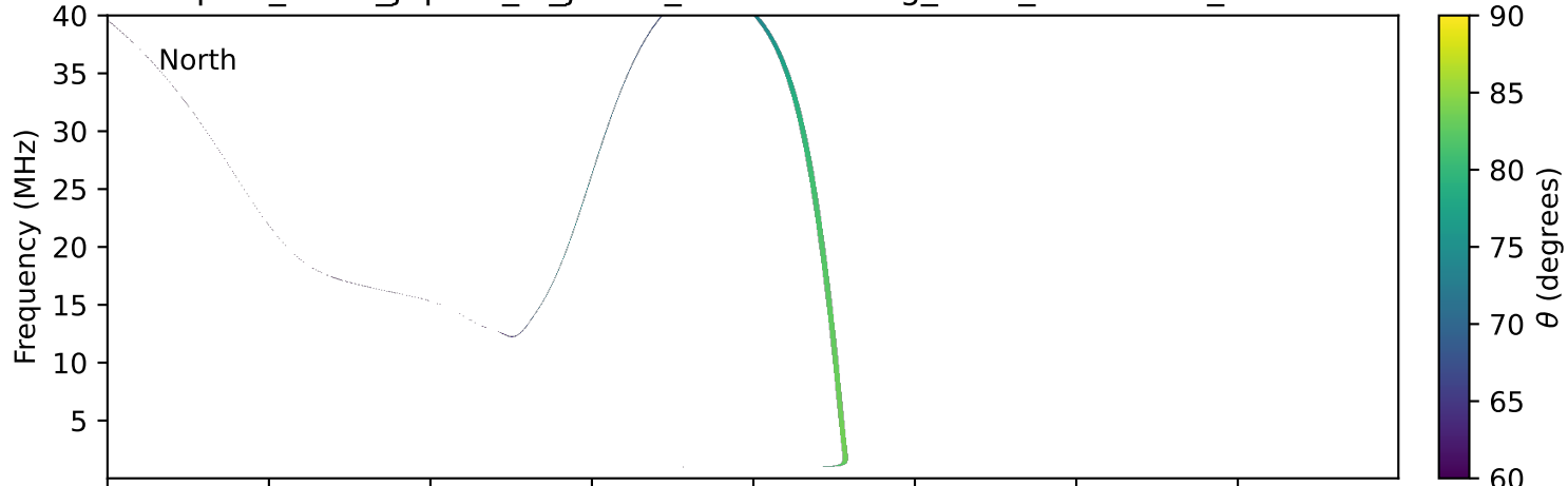
expres_earth_jupiter_io_jrm09_lossc-wid1deg_3kev_20000212_v11.cdf
