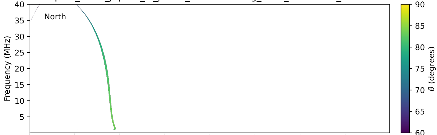
expres_earth_jupiter_io_jrm09_lossc-wid1deg_3kev_20000207_v11.cdf
