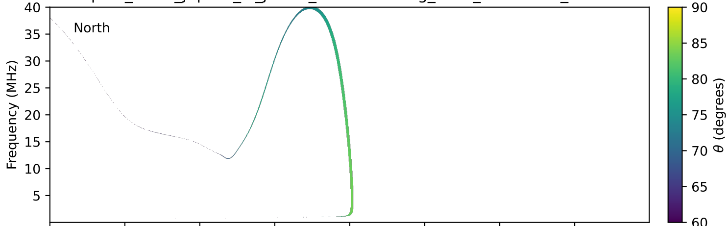
expres_earth_jupiter_io_jrm09_lossc-wid1deg_3kev_20000205_v11.cdf
