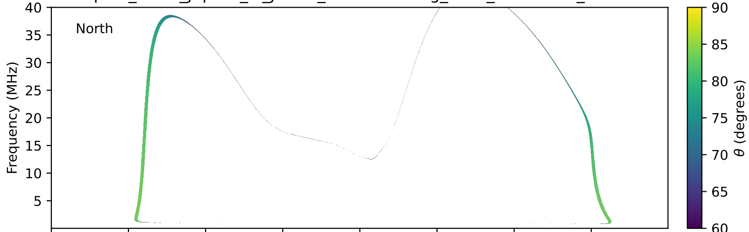
expres_earth_jupiter_io_jrm09_lossc-wid1deg_3kev_20000201_v11.cdf
