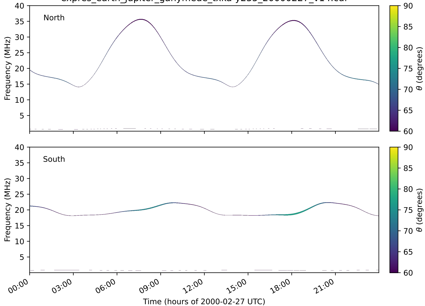
expres_earth_jupiter_ganymede_txka-y235_20000227_v14.cdf
