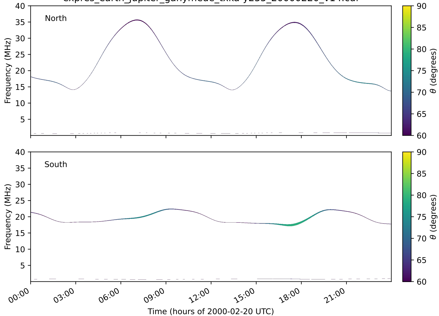
expres_earth_jupiter_ganymede_txka-y235_20000220_v14.cdf
