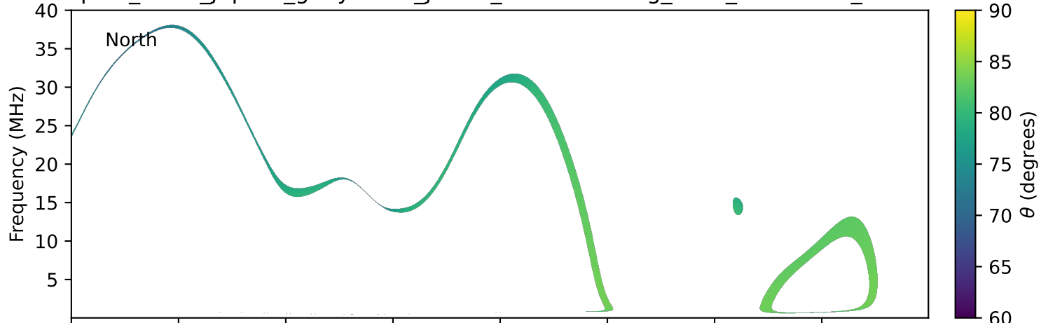
expres_earth_jupiter_ganymede_jrm33_lossc-wid1deg_3kev_20000207_v11.cdf
