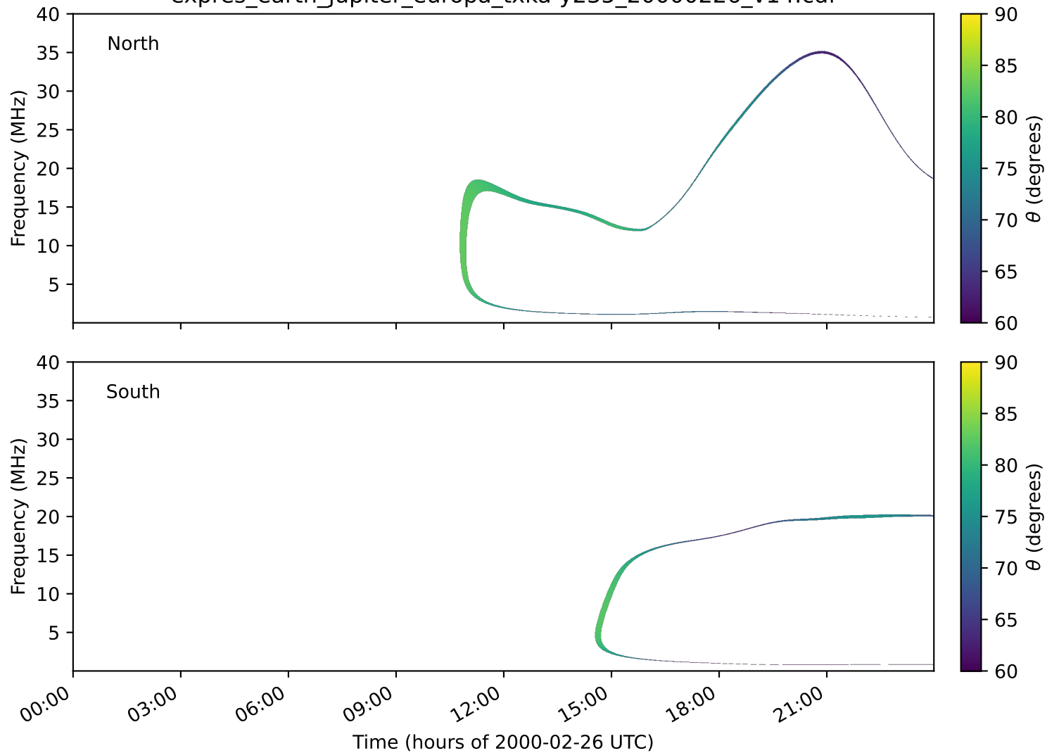
expres_earth_jupiter_europa_txka-y235_20000226_v14.cdf
