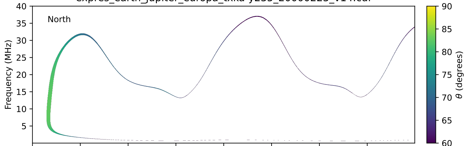
expres_earth_jupiter_europa_txka-y235_20000223_v14.cdf
