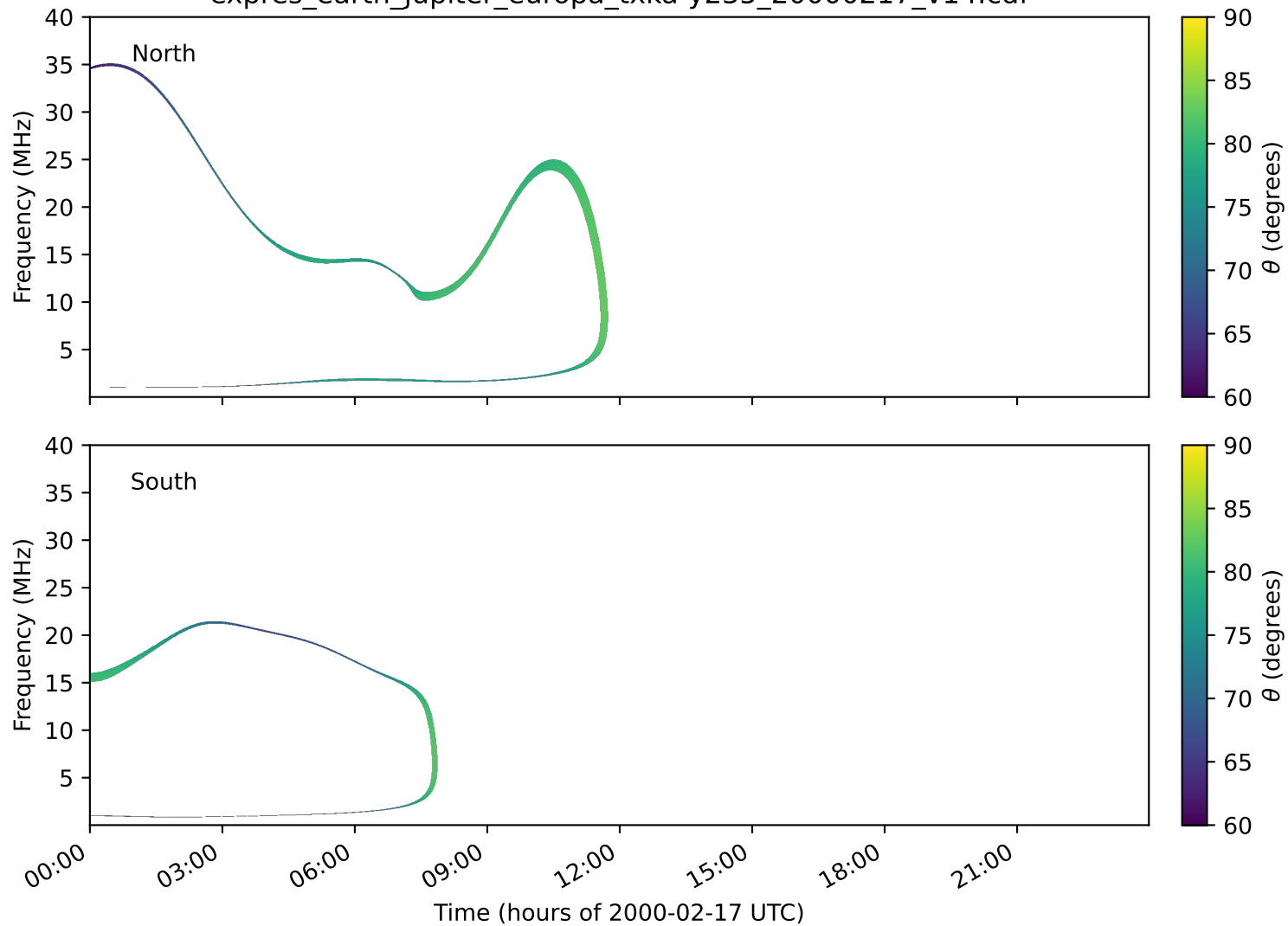
expres_earth_jupiter_europa_txka-y235_20000217_v14.cdf
