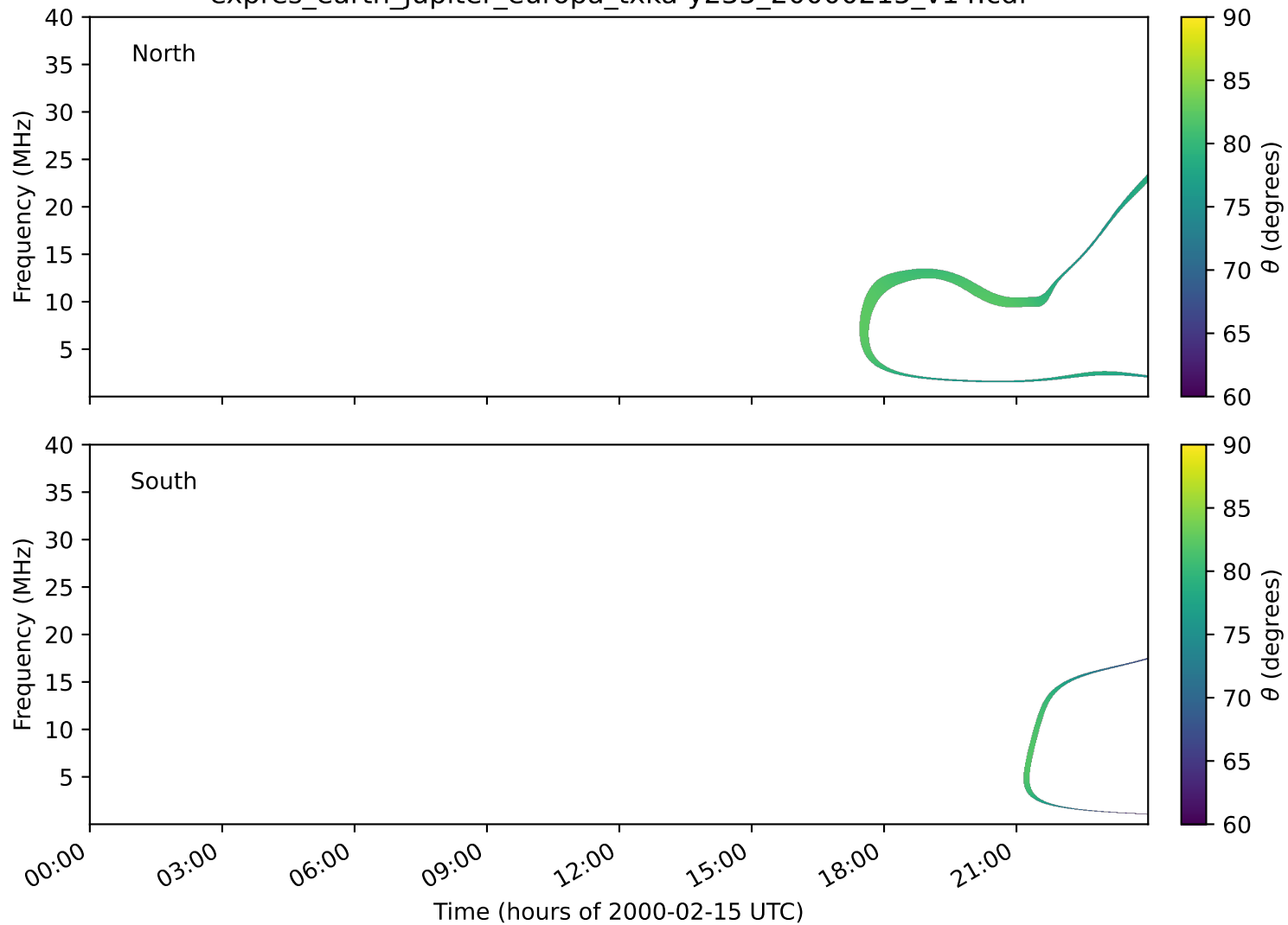
expres_earth_jupiter_europa_txka-y235_20000215_v14.cdf
