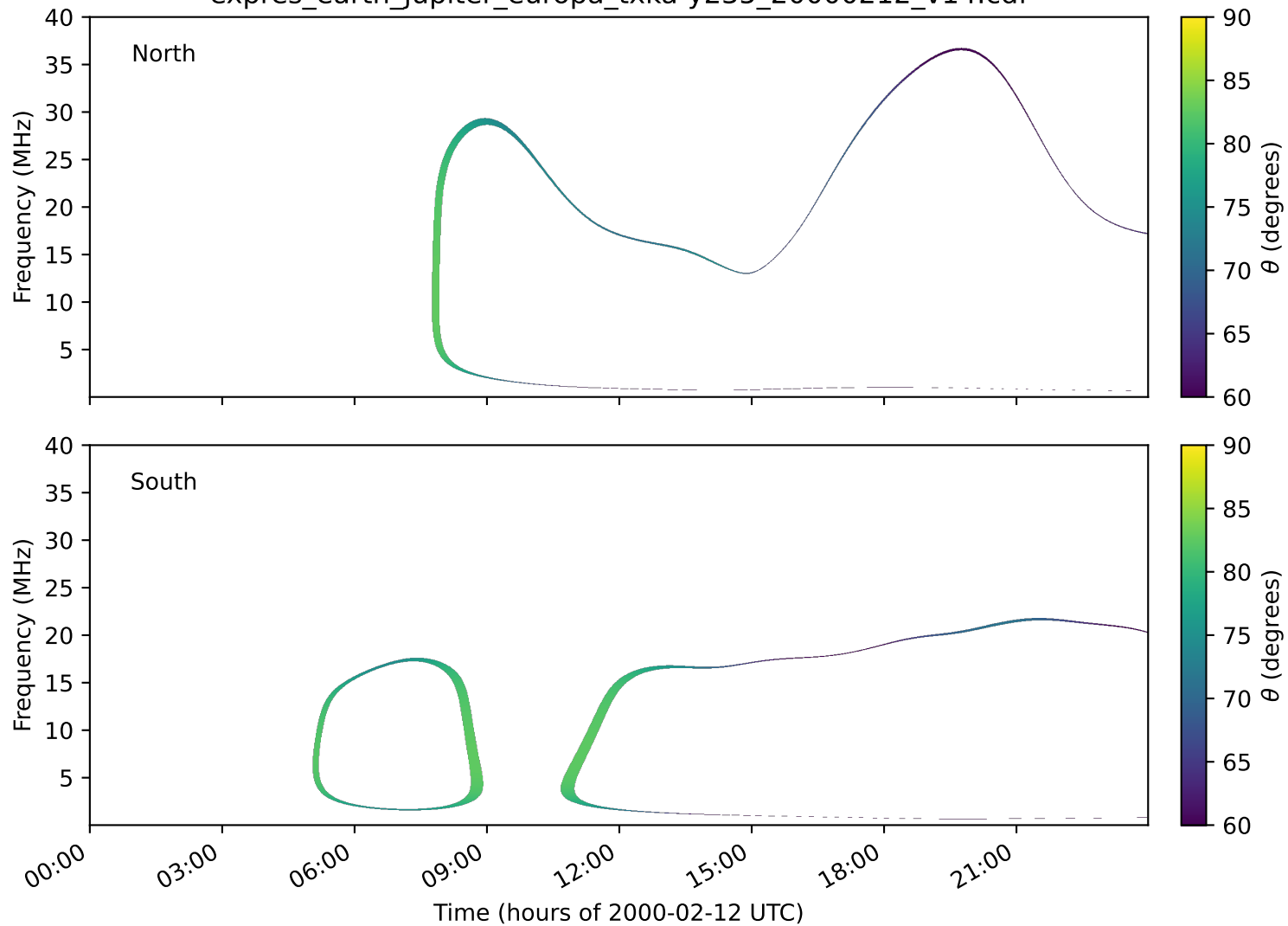
expres_earth_jupiter_europa_txka-y235_20000212_v14.cdf
