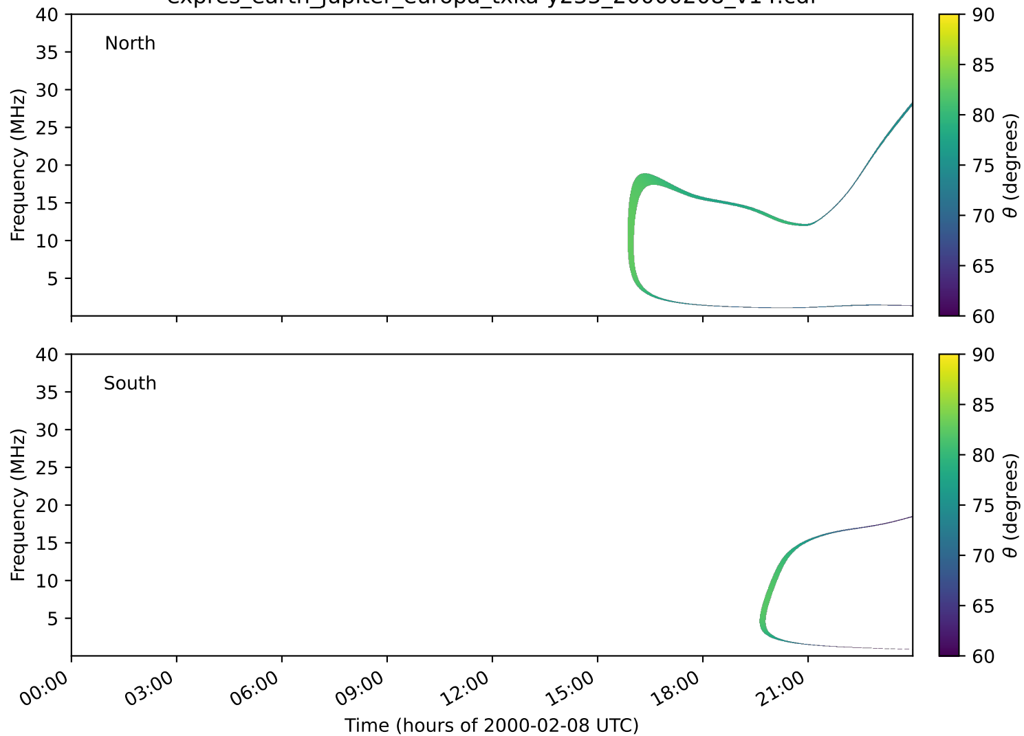
expres_earth_jupiter_europa_txka-y235_20000208_v14.cdf
