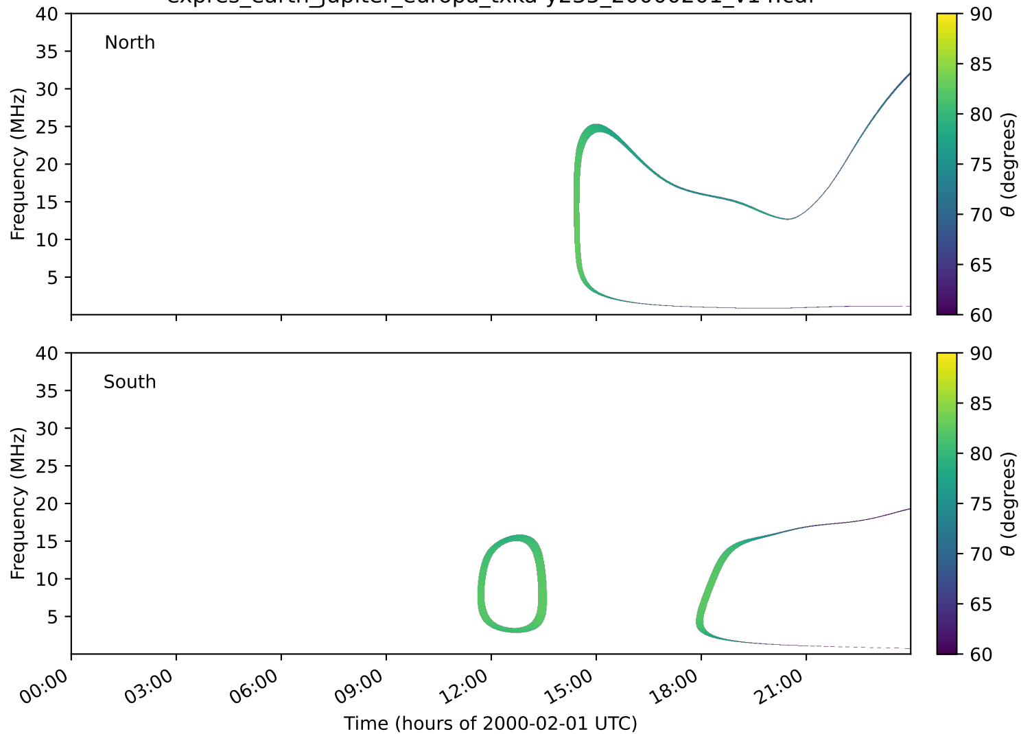
expres_earth_jupiter_europa_txka-y235_20000201_v14.cdf
