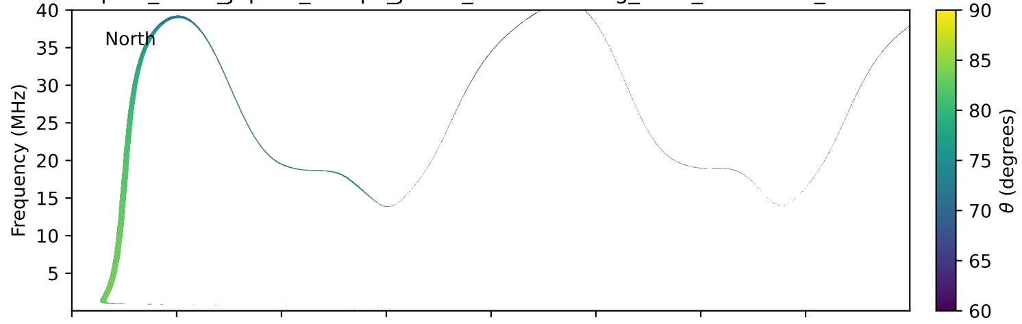
expres_earth_jupiter_europa_jrm33_lossc-wid1deg_3kev_20000223_v11.cdf
