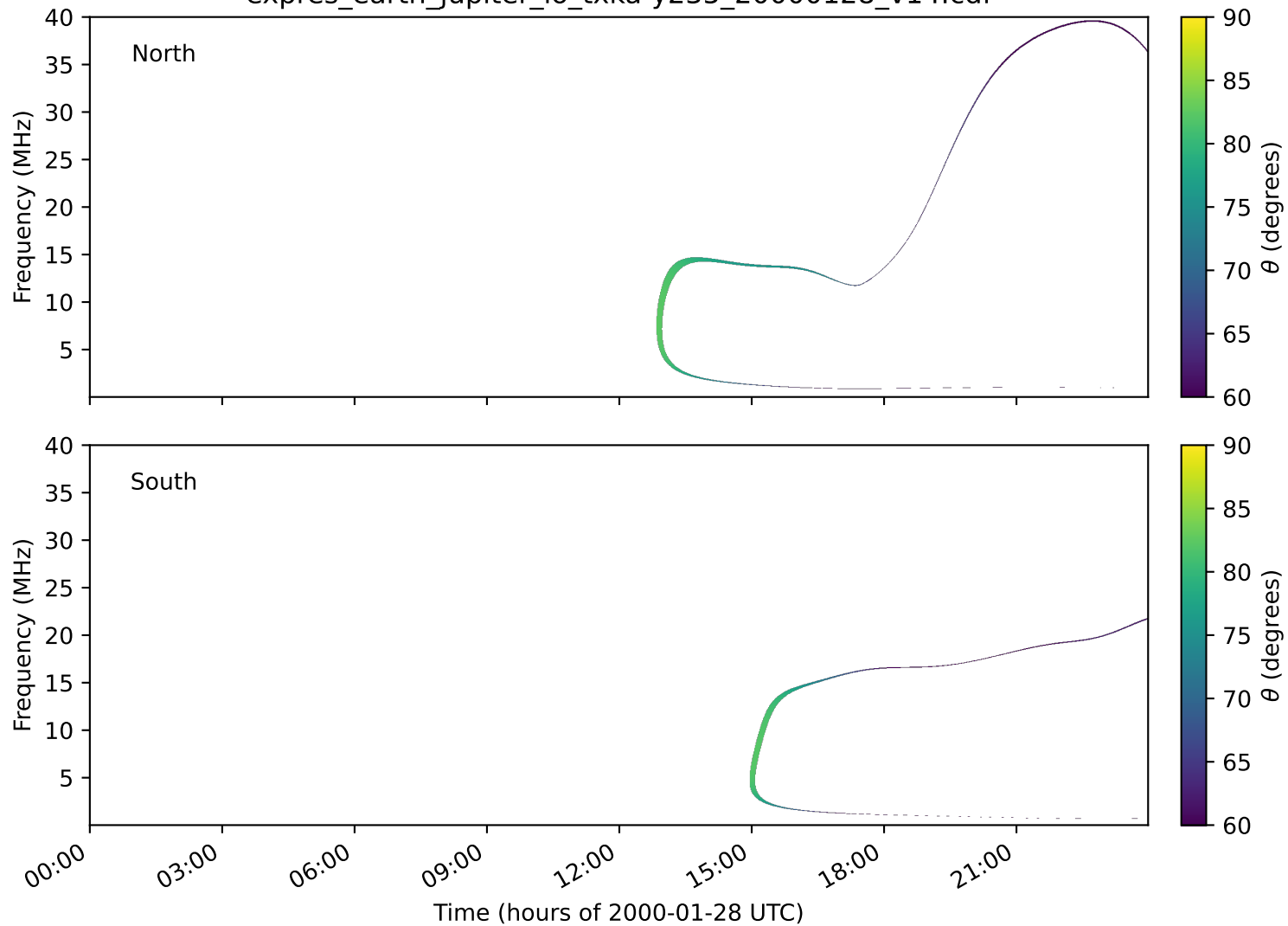
expres_earth_jupiter_io_txka-y235_20000128_v14.cdf
