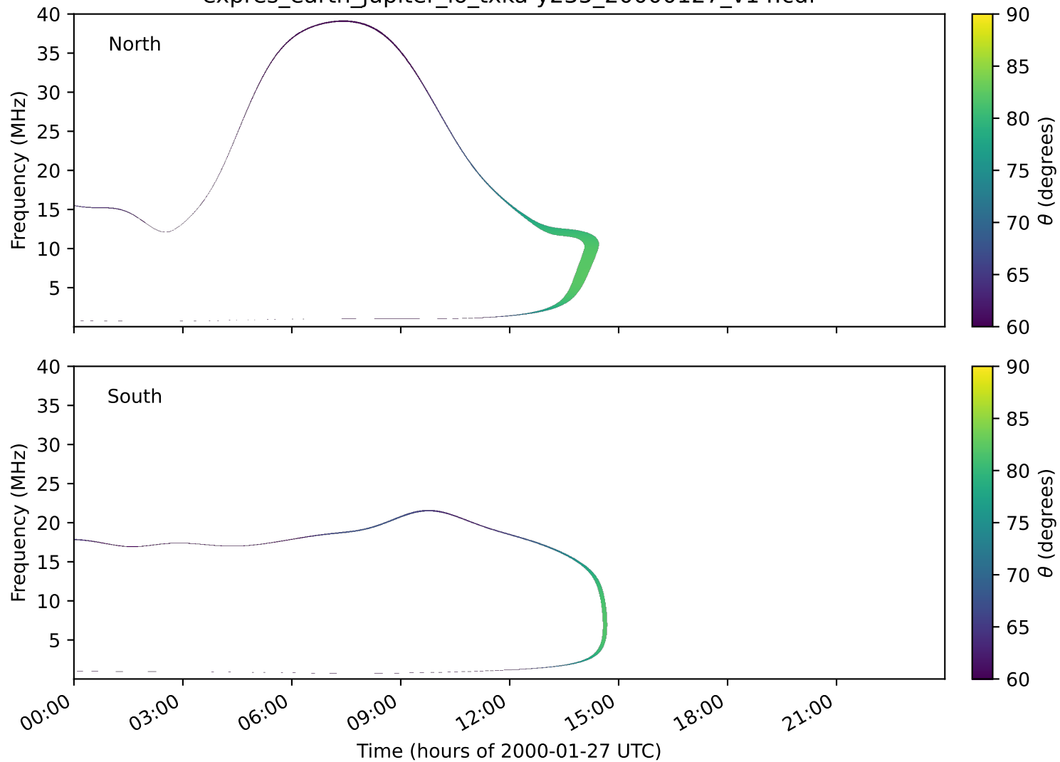
expres_earth_jupiter_io_txka-y235_20000127_v14.cdf
