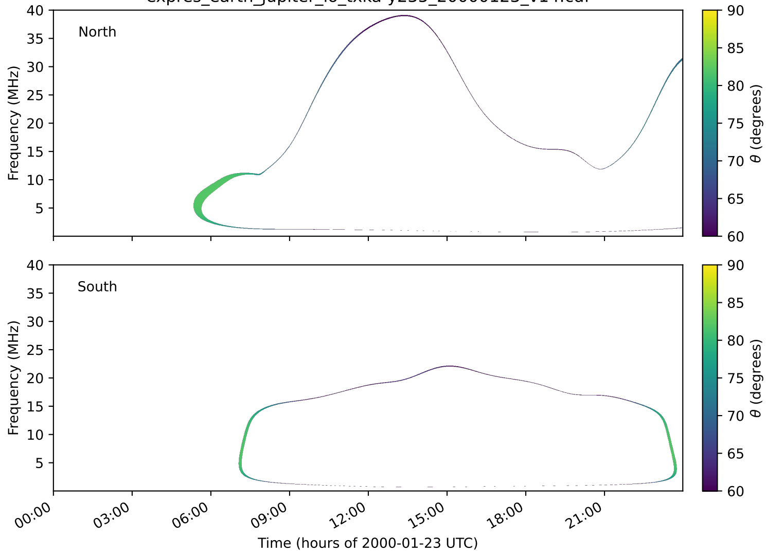
expres_earth_jupiter_io_txka-y235_20000123_v14.cdf
